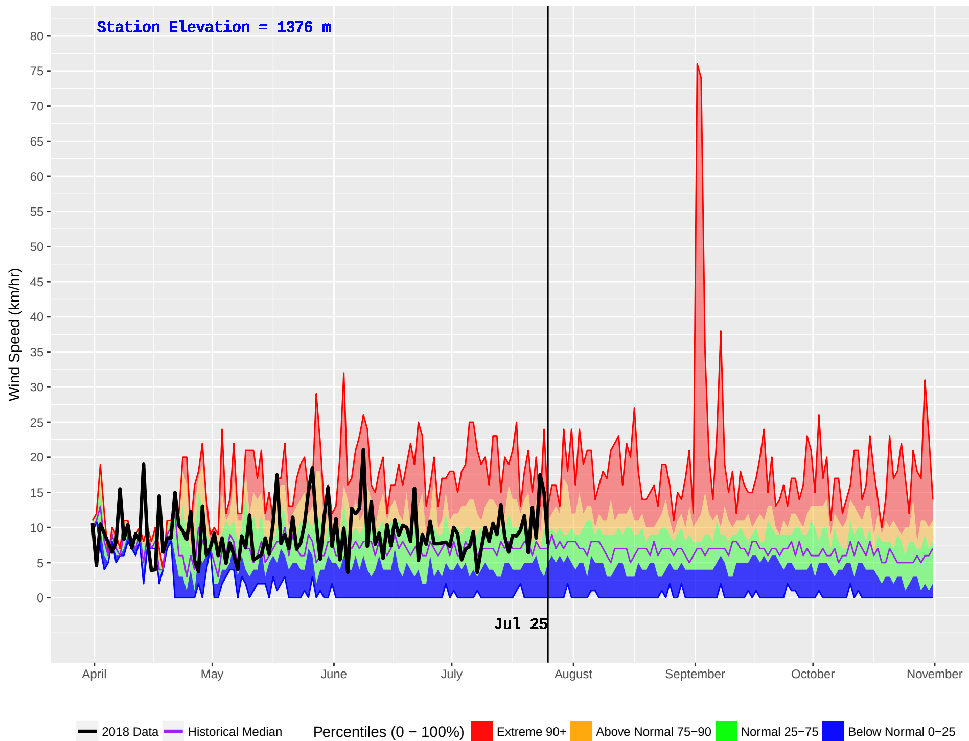
DUNCAN (385) : Historical (1981–2016) and Current (2018) Noon Wind Speed
