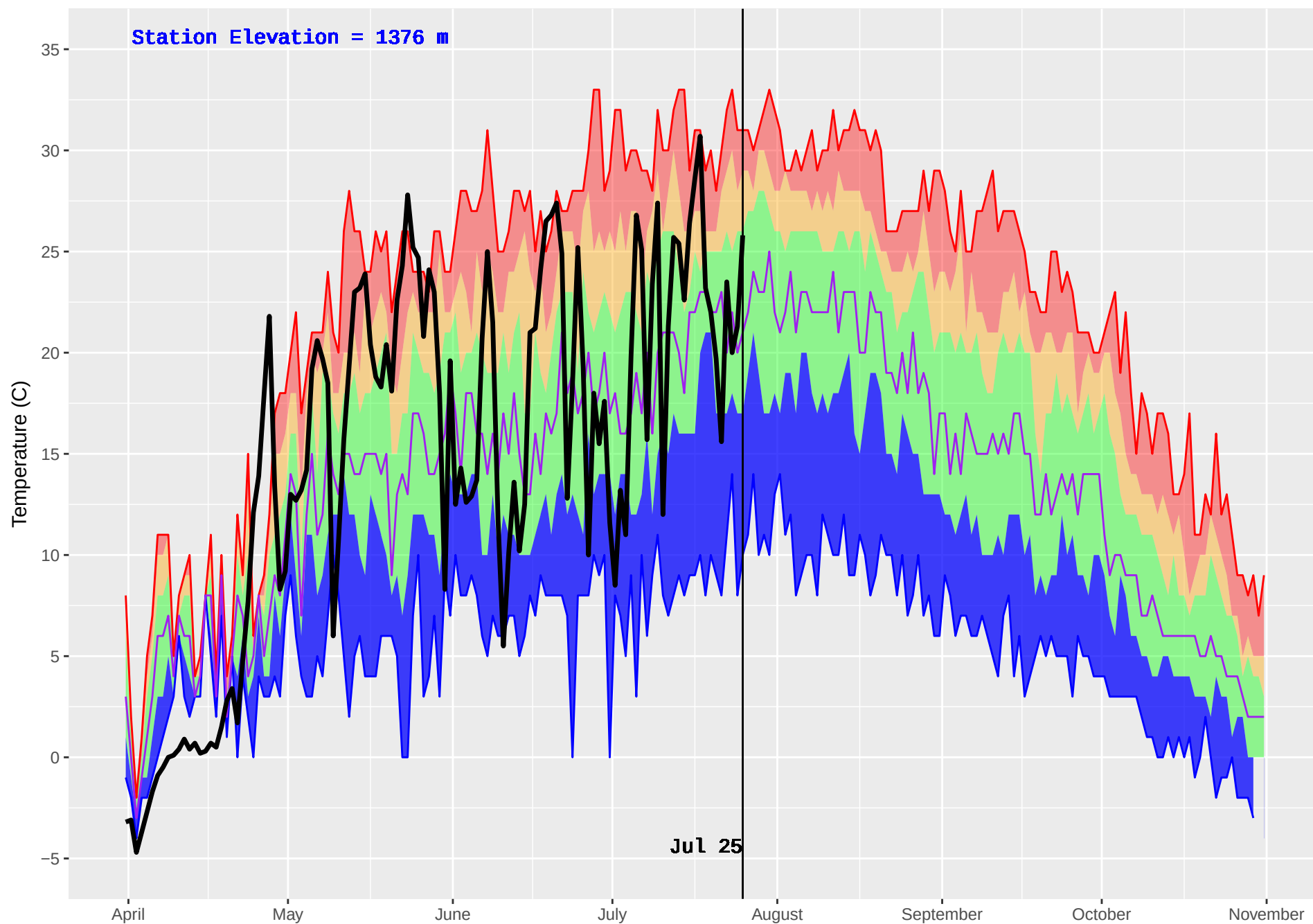
DUNCAN (385) : Historical (1981–2016) and Current (2018) Noon Temperature
