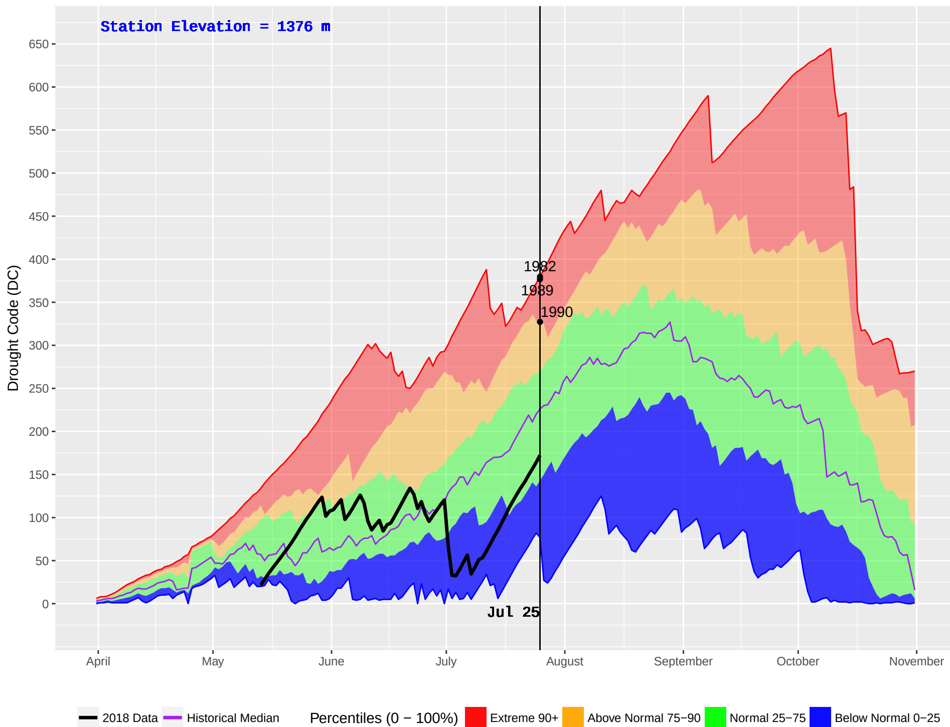
DUNCAN (385) : Historical (1981–2016) and Current (2018) Noon Drought Code (DC)
